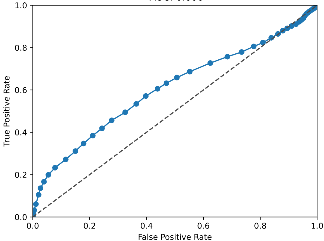
EGR1 ROC Curve AUC: 0.606
