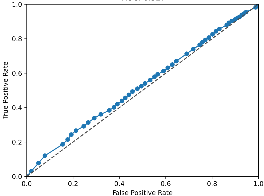
NFKB1 ROC Curve AUC: 0.527
