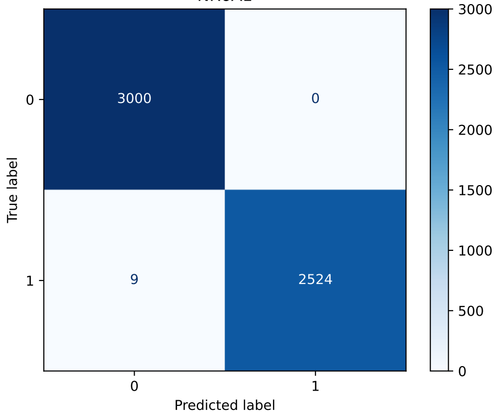
NR6A1
