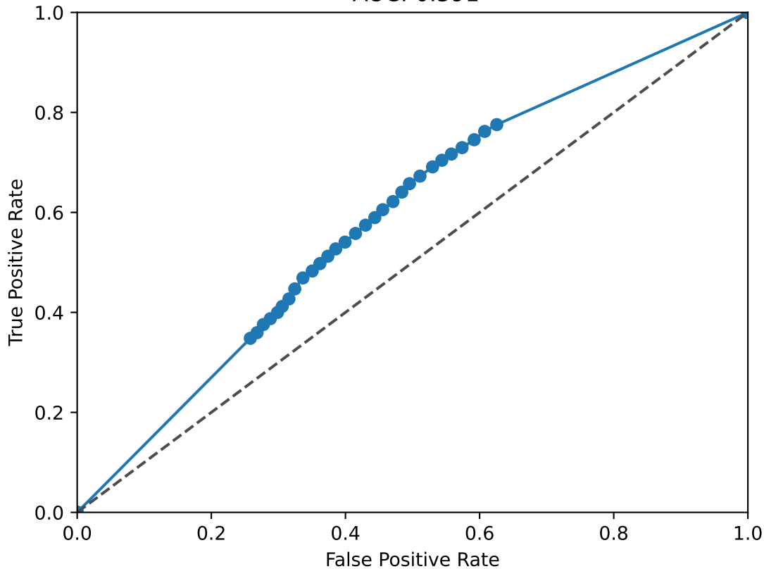
THRB ROC Curve AUC: 0.591
