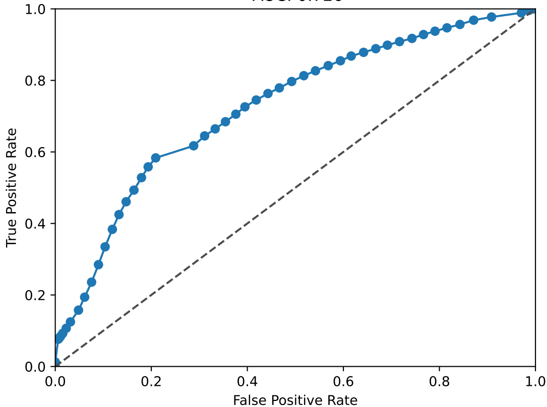
FOS ROC Curve AUC: 0.726
