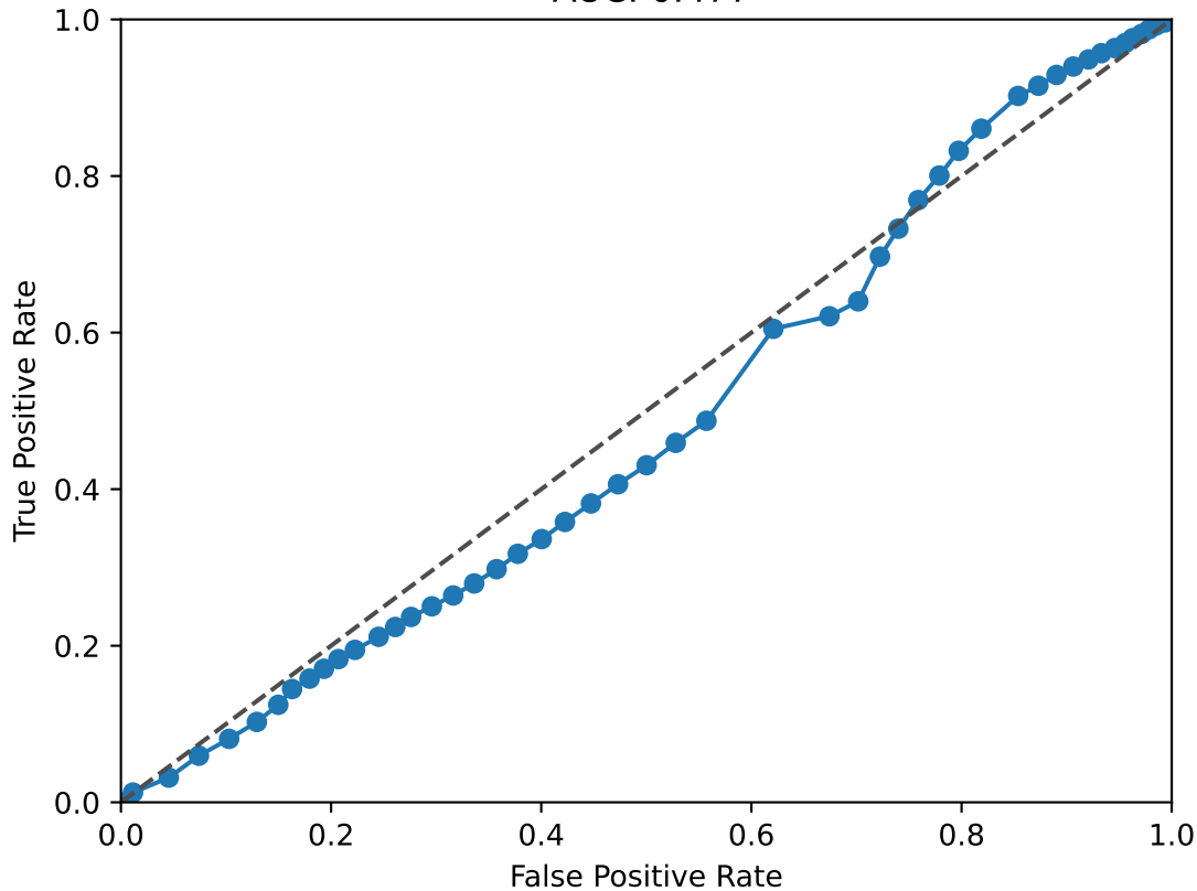
GRHL2 ROC Curve AUC: 0.477
