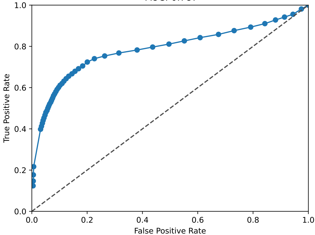
NFIX ROC Curve AUC: 0.787
