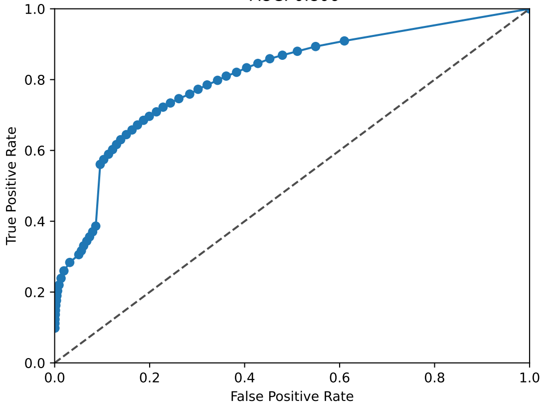
REST ROC Curve AUC: 0.806
