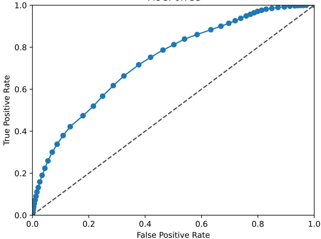
SIX4 ROC Curve AUC: 0.735
