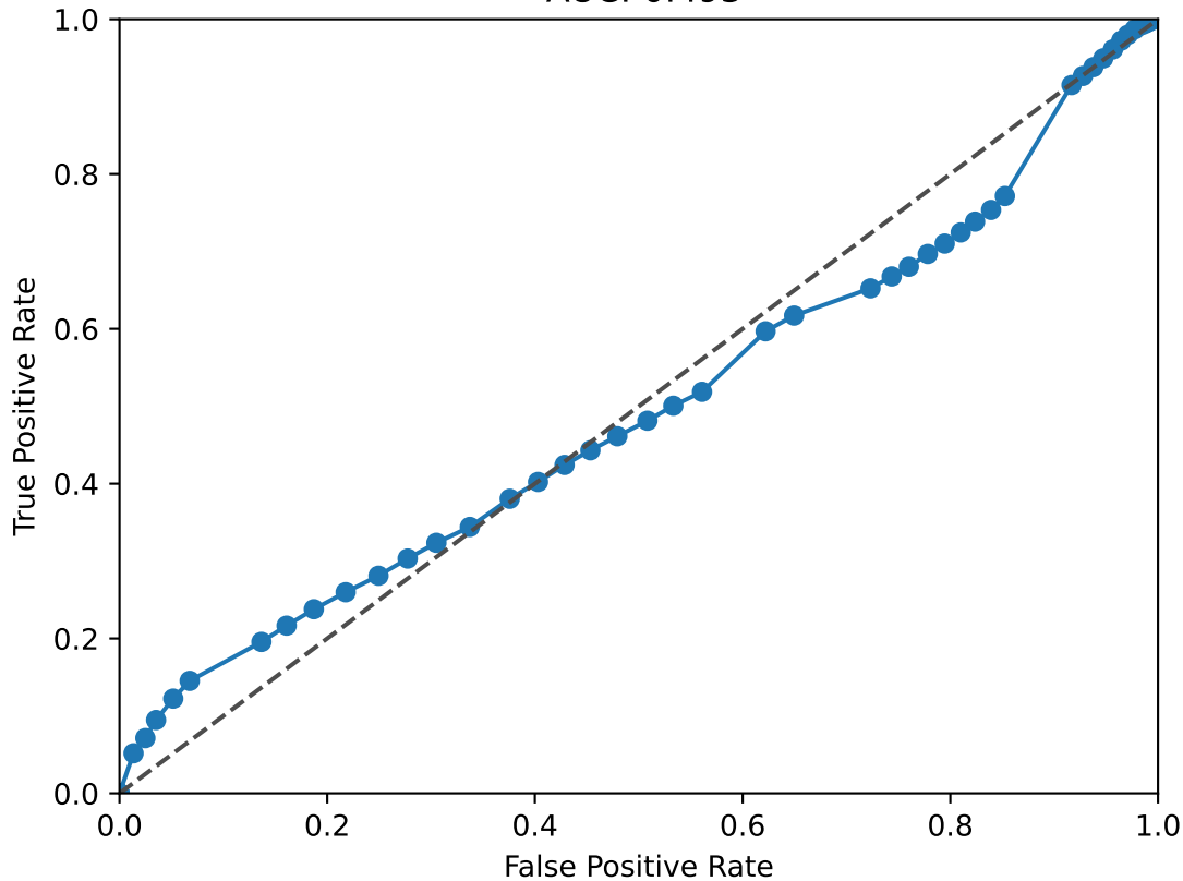
JUNB ROC Curve AUC: 0.493
