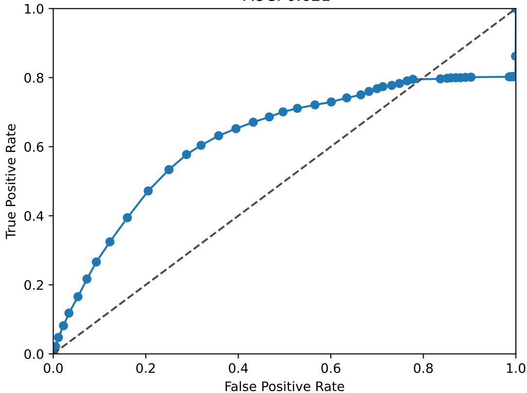
EGR1 ROC Curve AUC: 0.621
