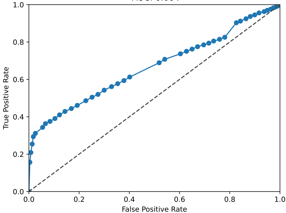
JUNB ROC Curve AUC: 0.664
