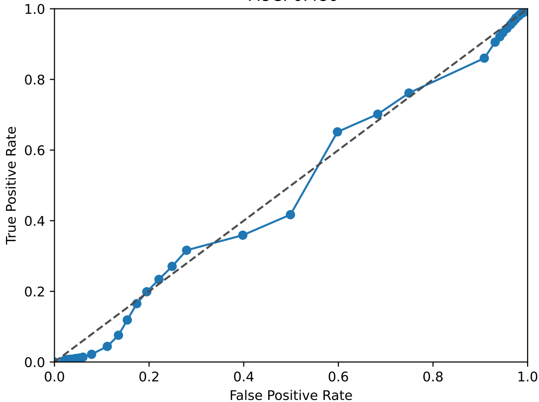
PBX1 ROC Curve AUC: 0.486
