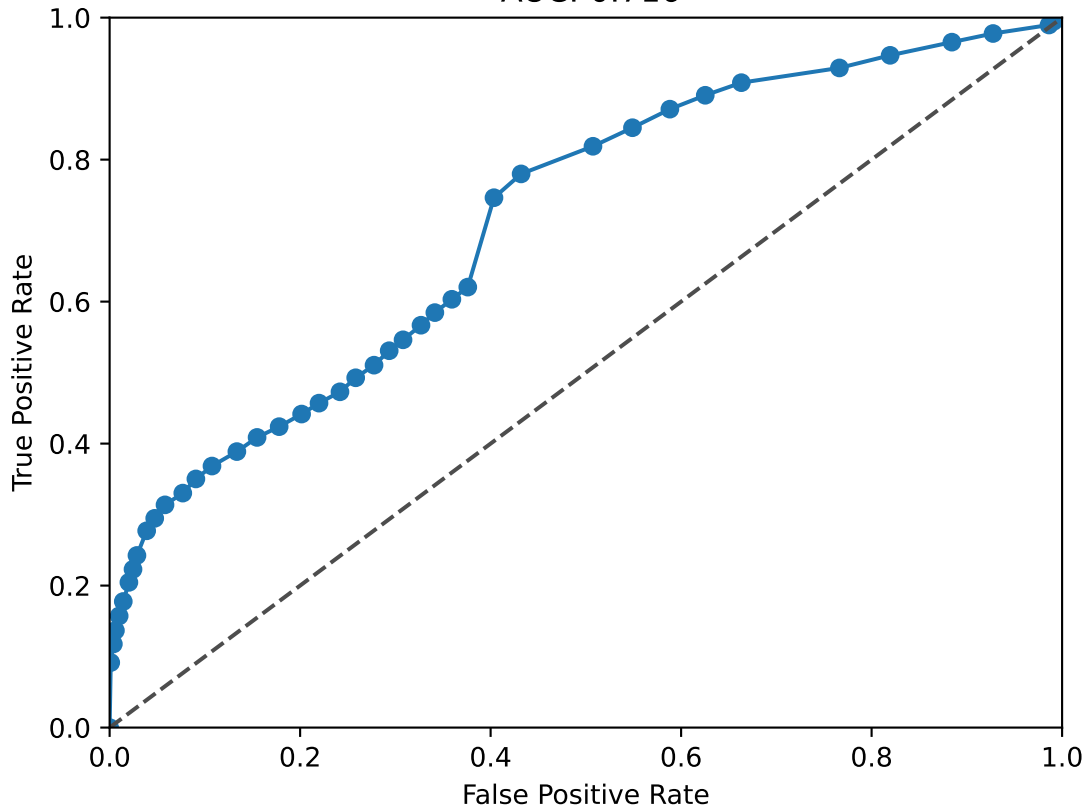
BACH2 ROC Curve
