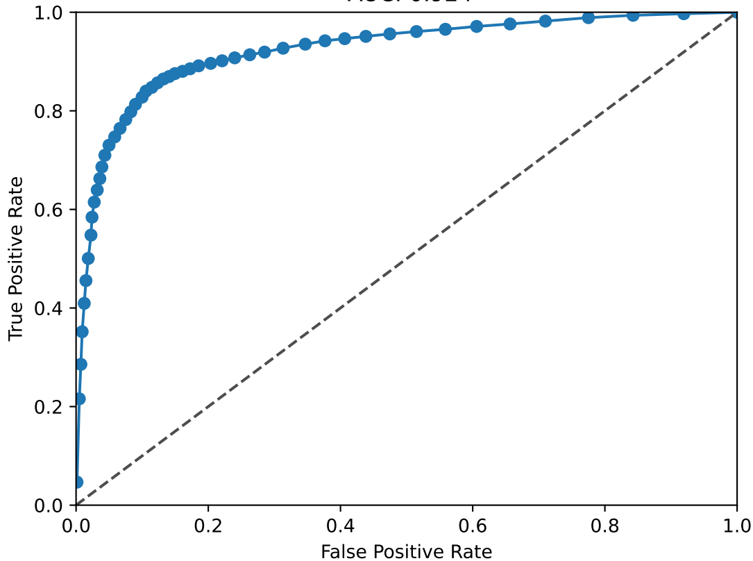
NCAM1 ROC Curve
