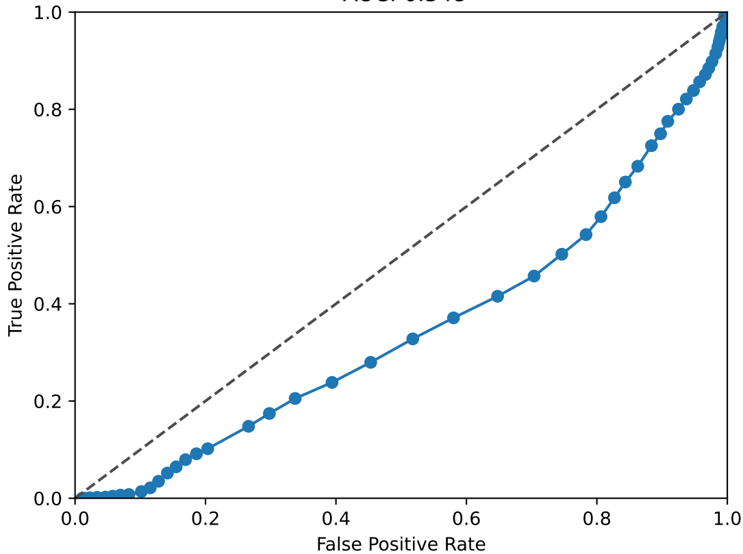
NFIA ROC Curve AUC: 0.348
