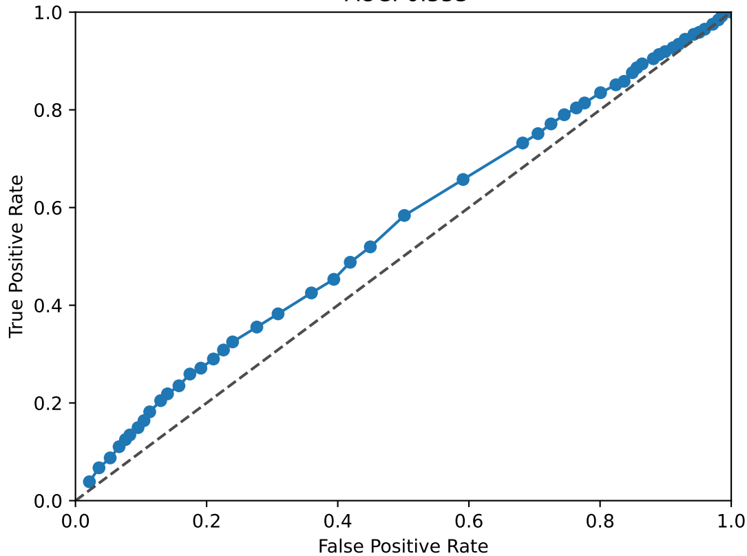
CUX2 ROC Curve AUC: 0.553
