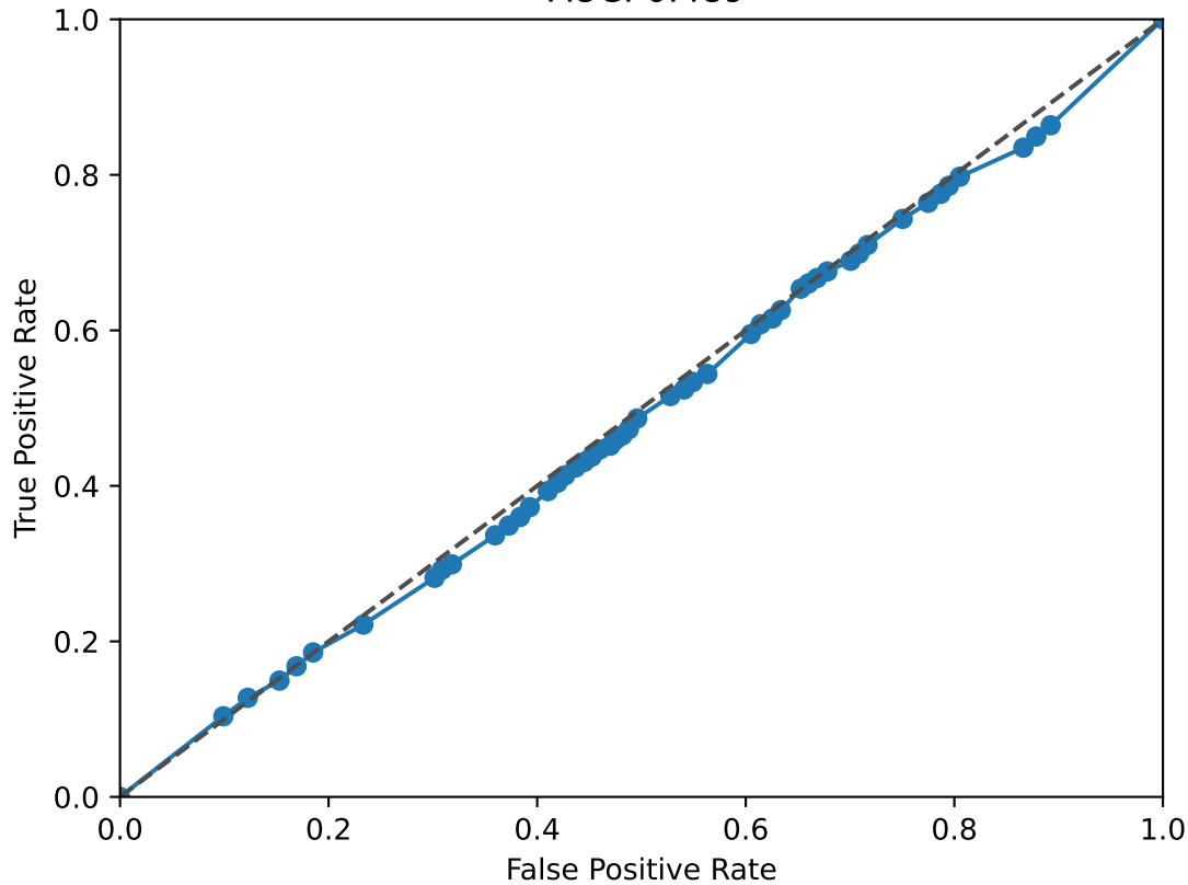
GRHL2 ROC Curve AUC: 0.489
