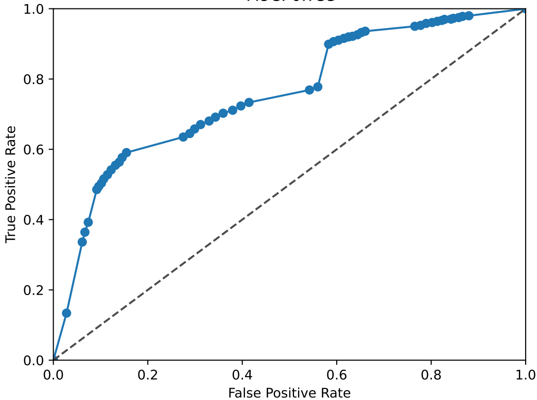
JUNB ROC Curve AUC: 0.755
