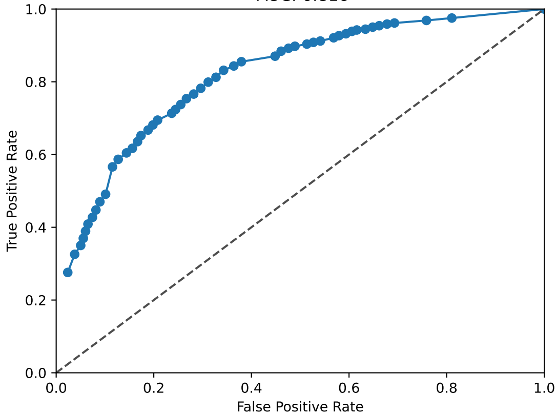
JUN ROC Curve AUC: 0.816
