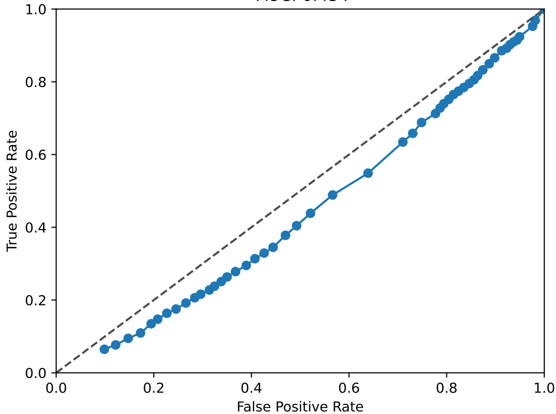
NCAM1 ROC Curve AUC: 0.434
