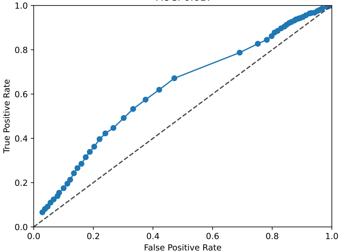
SIX4 ROC Curve AUC: 0.617
