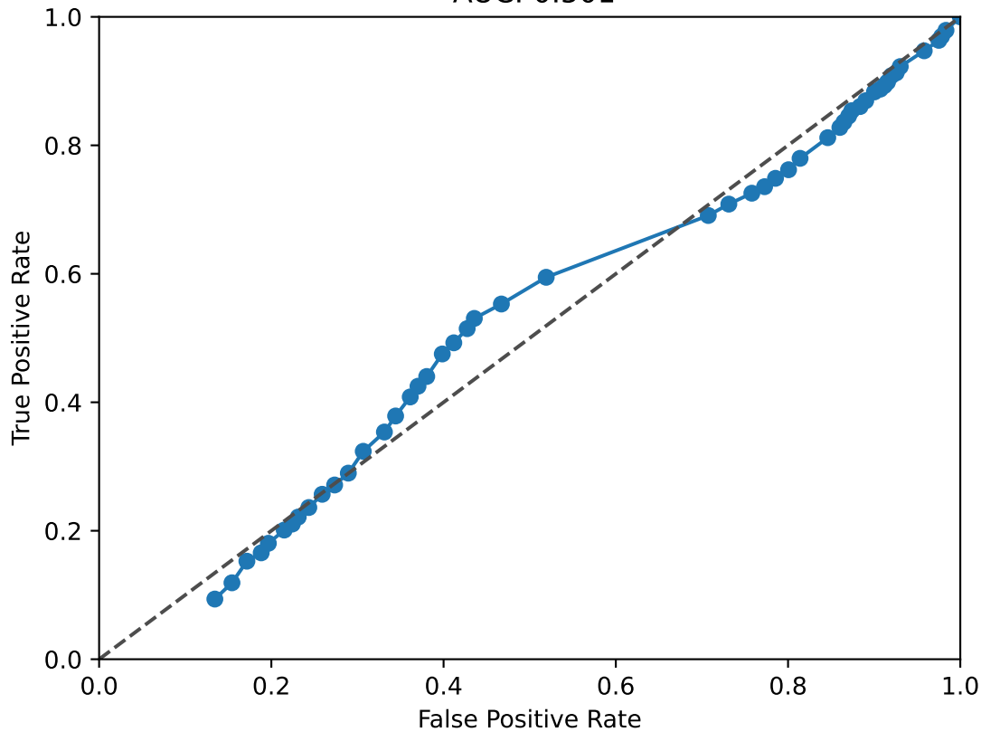
TBX15 ROC Curve AUC: 0.501
