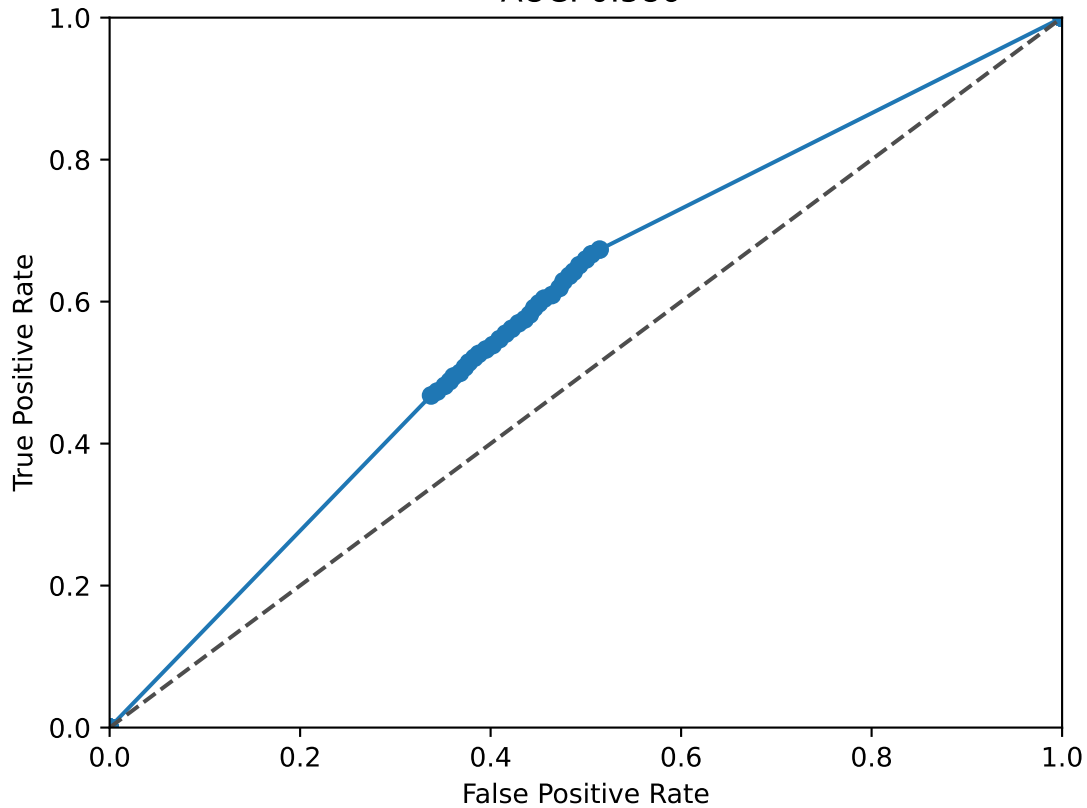
THR B ROC Curve AUC: 0.586
