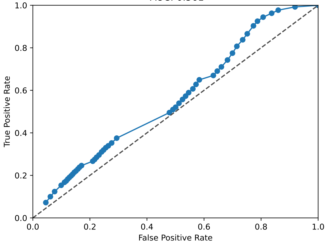
ASCL1 ROC Curve AUC: 0.561
