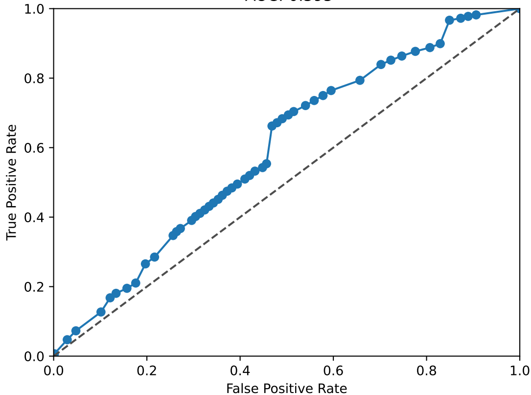
BACH1 ROC Curve AUC: 0.595
