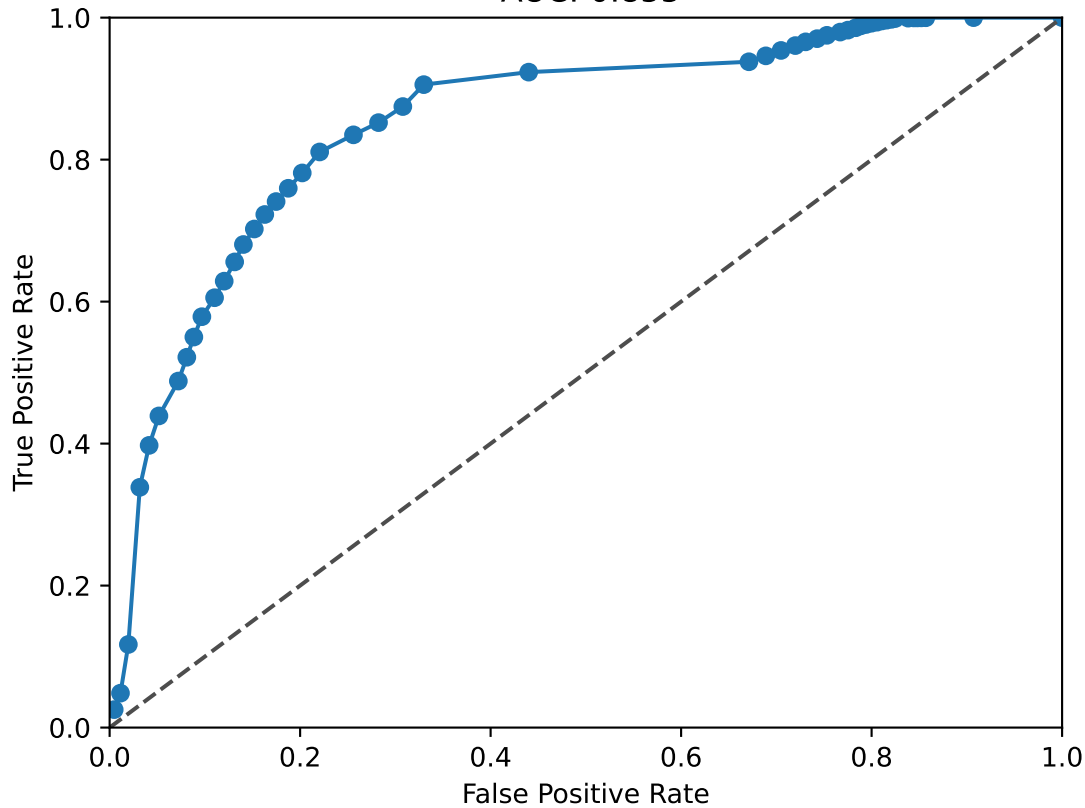
CUX2 ROC Curve AUC: 0.855
