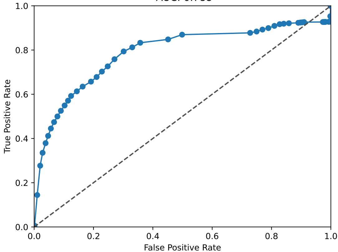
EGR1 ROC Curve AUC: 0.788
