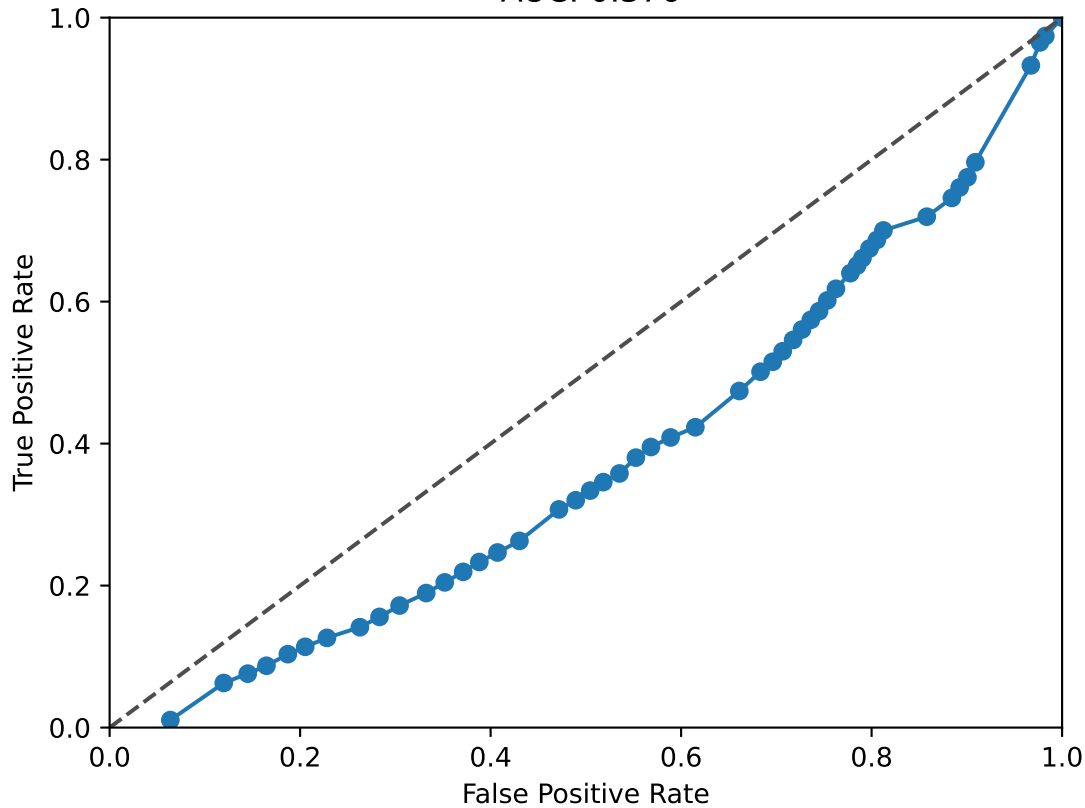
EPCAM ROC Curve AUC: 0.376
