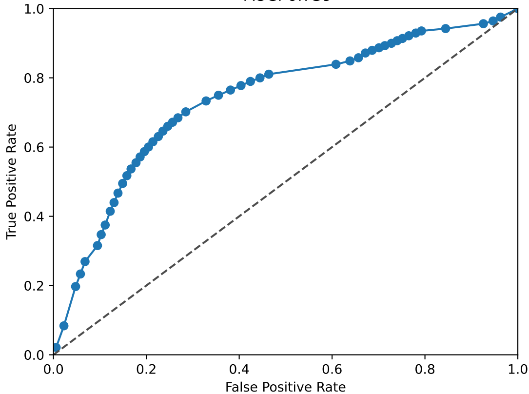
FOS ROC Curve AUC: 0.739
