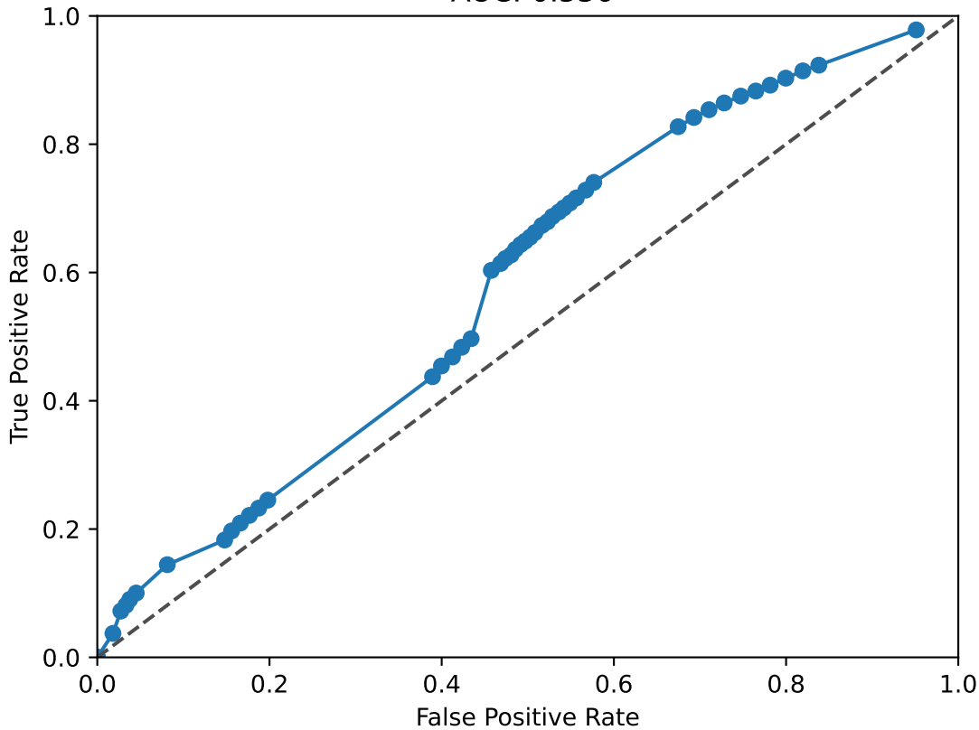
FOXO3 ROC Curve AUC: 0.536
