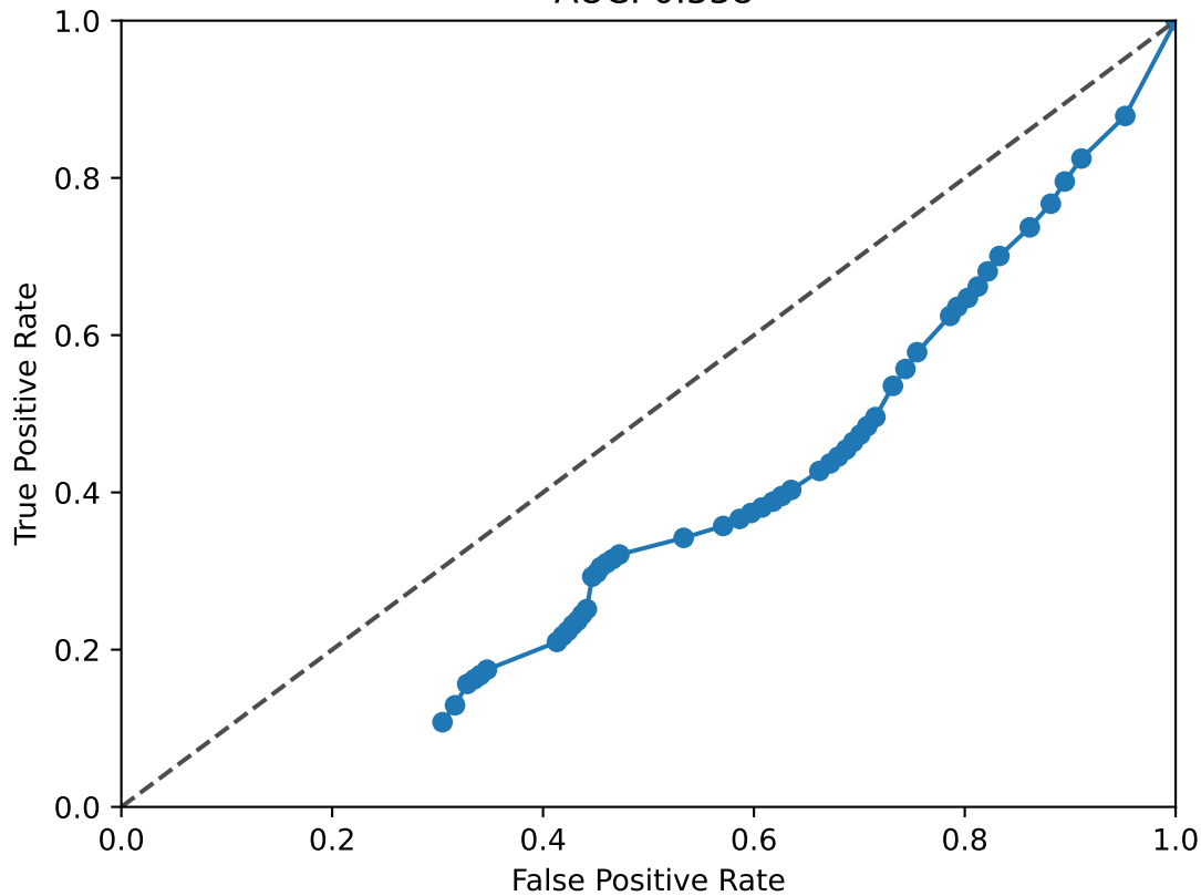
HES1 ROC Curve AUC: 0.338
