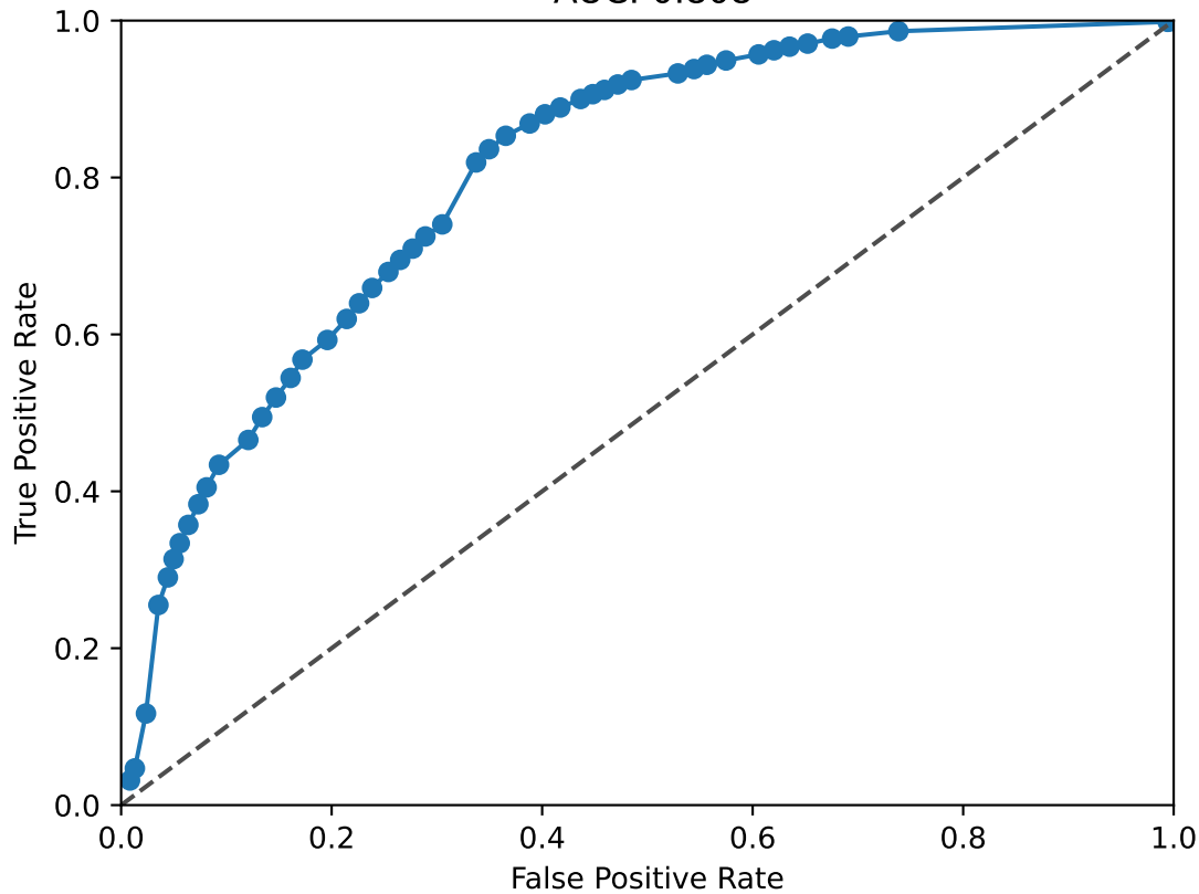
HSF2 ROC Curve AUC: 0.808
