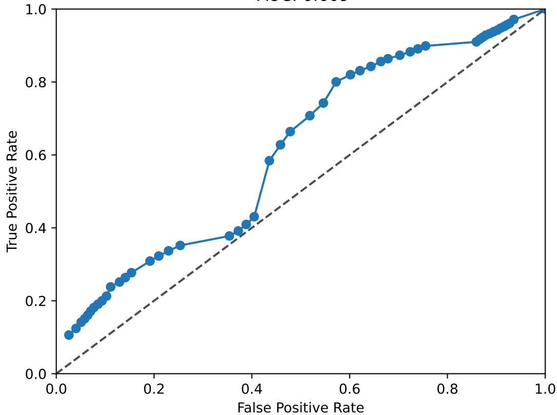
JUN ROC Curve AUC: 0.609
