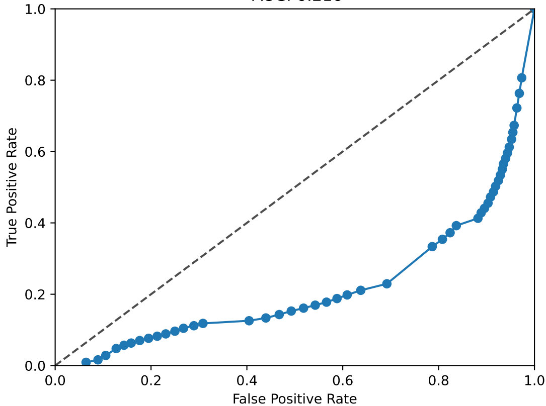
NFIB ROC Curve AUC: 0.216
