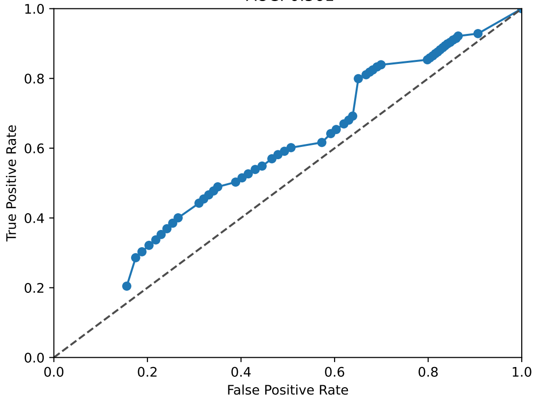
RORA_RORB ROC Curve AUC: 0.561
