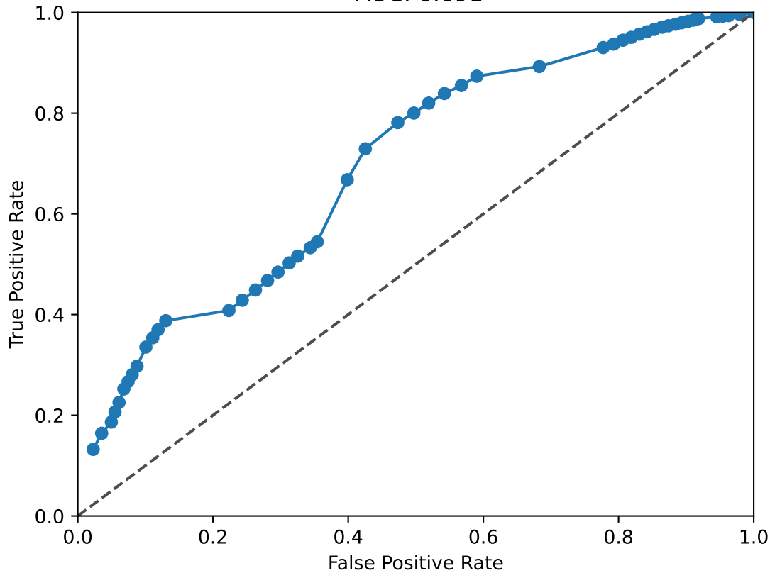
TBX15 ROC Curve AUC: 0.691
