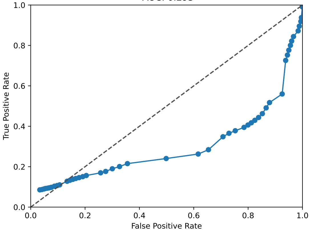
TCF7L1 ROC Curve AUC: 0.293
