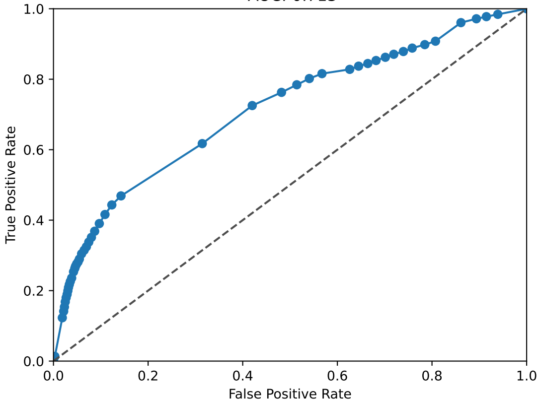
TEAD1 ROC Curve AUC: 0.713
