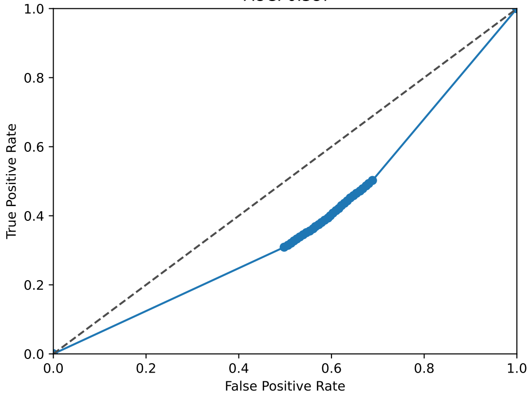
THRB ROC Curve AUC: 0.387
