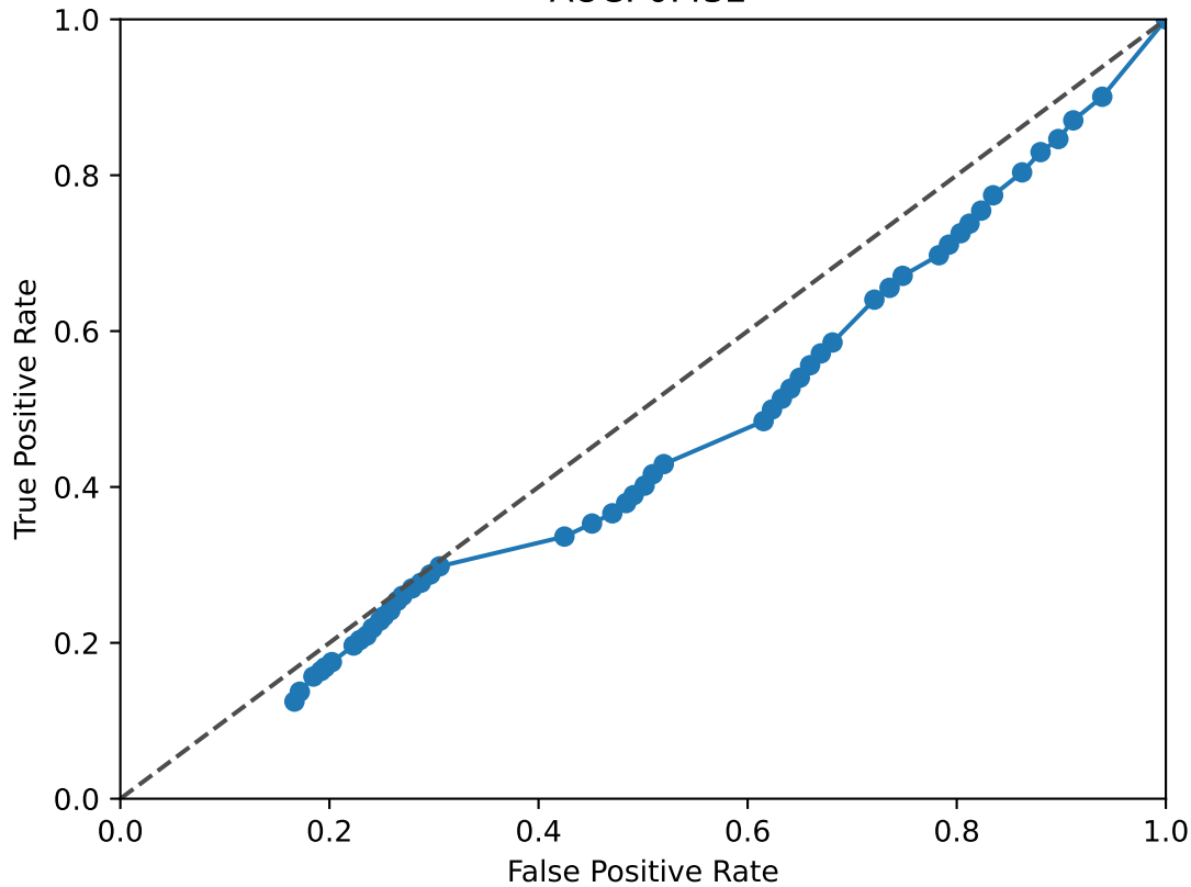
HES1 ROC Curve AUC: 0.432
