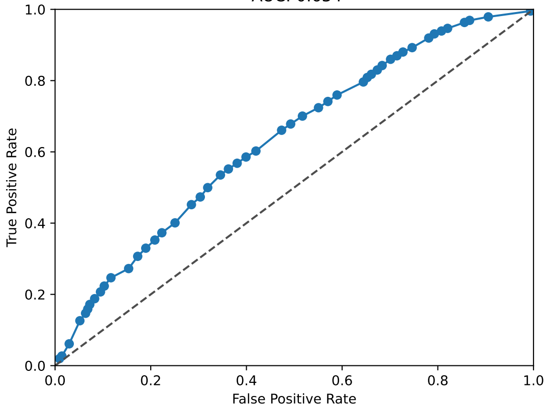
HSF2 ROC Curve AUC: 0.634
