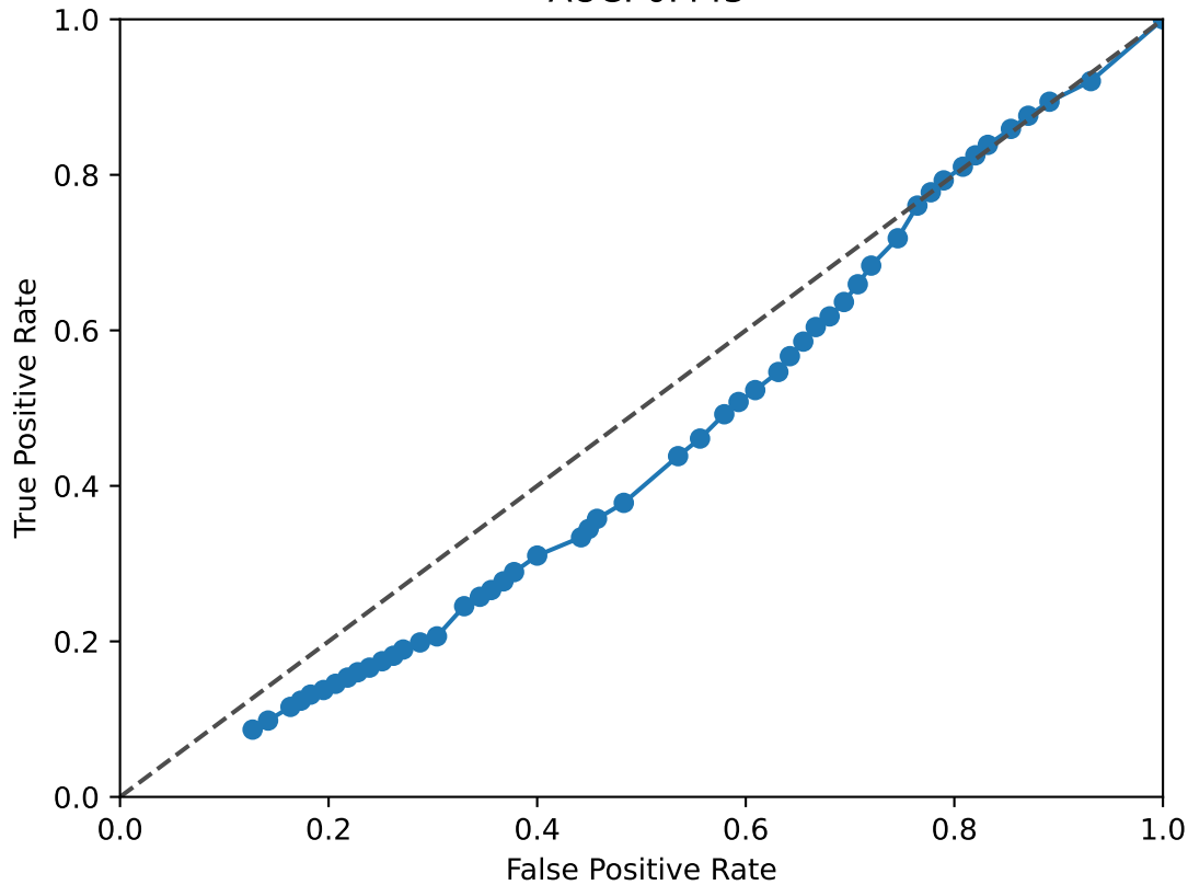
ICAM1 ROC Curve AUC: 0.443
