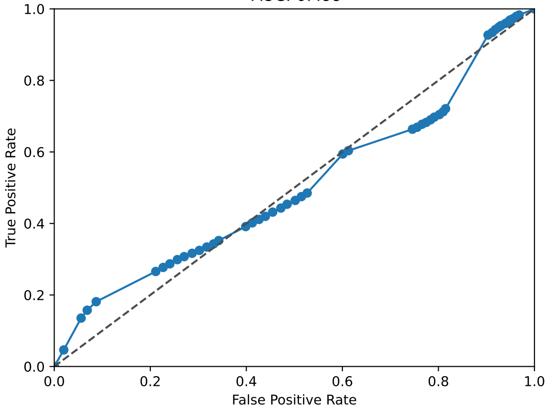
JUNB ROC Curve AUC: 0.499
