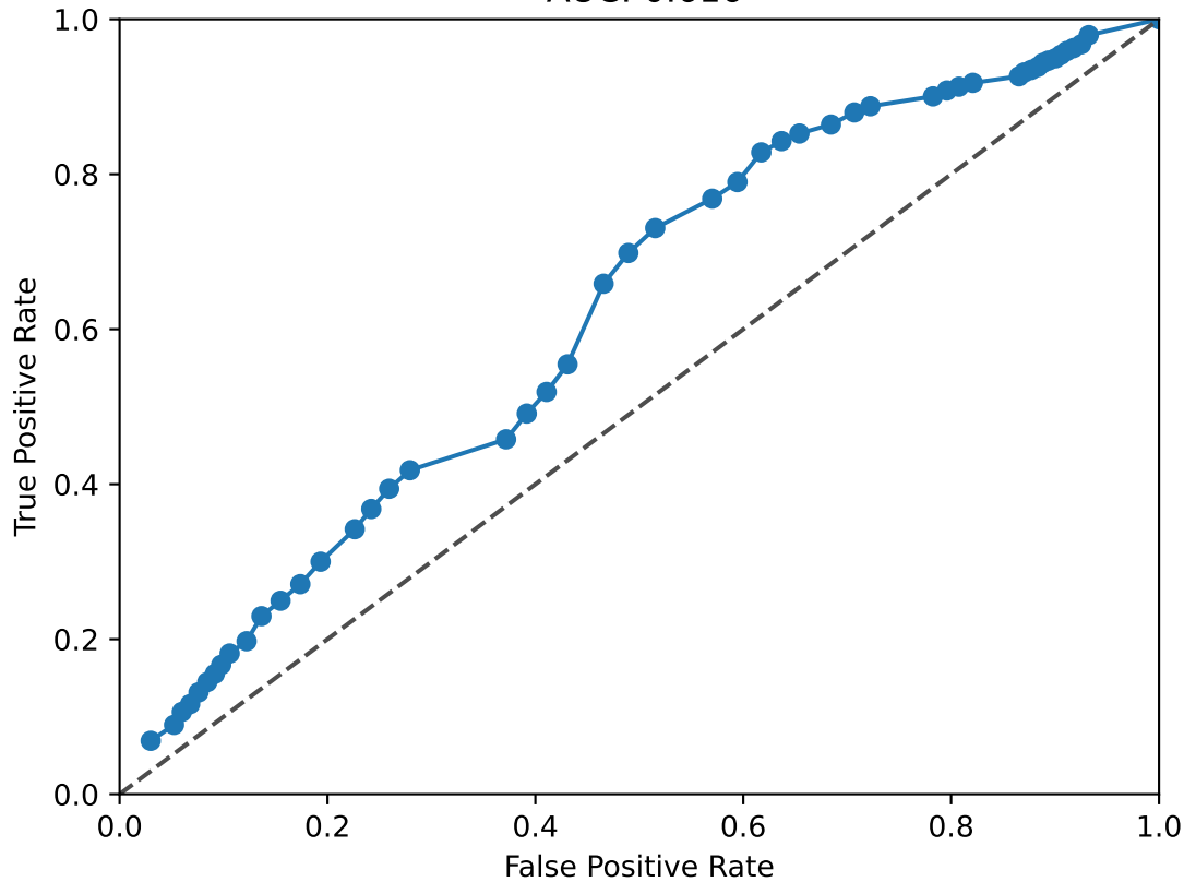
JUN ROC Curve AUC: 0.616
