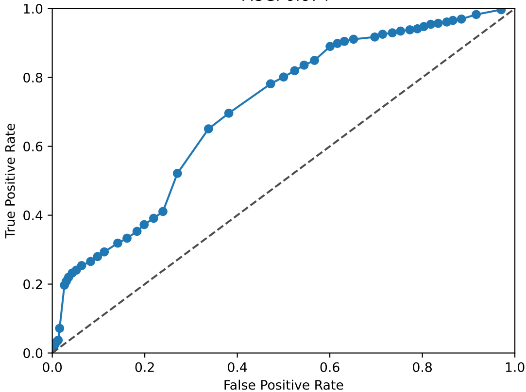
NFIA ROC Curve AUC: 0.674
