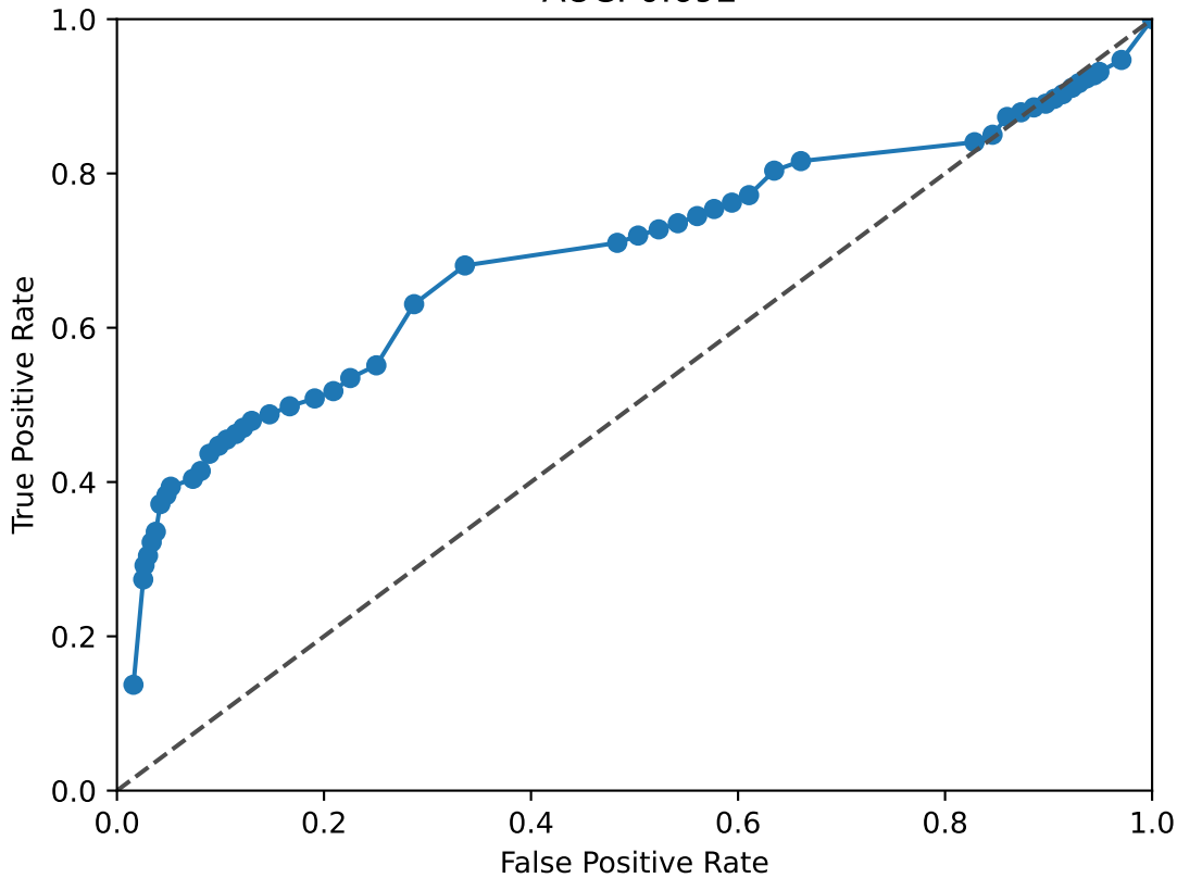
NFIX ROC Curve AUC: 0.692
