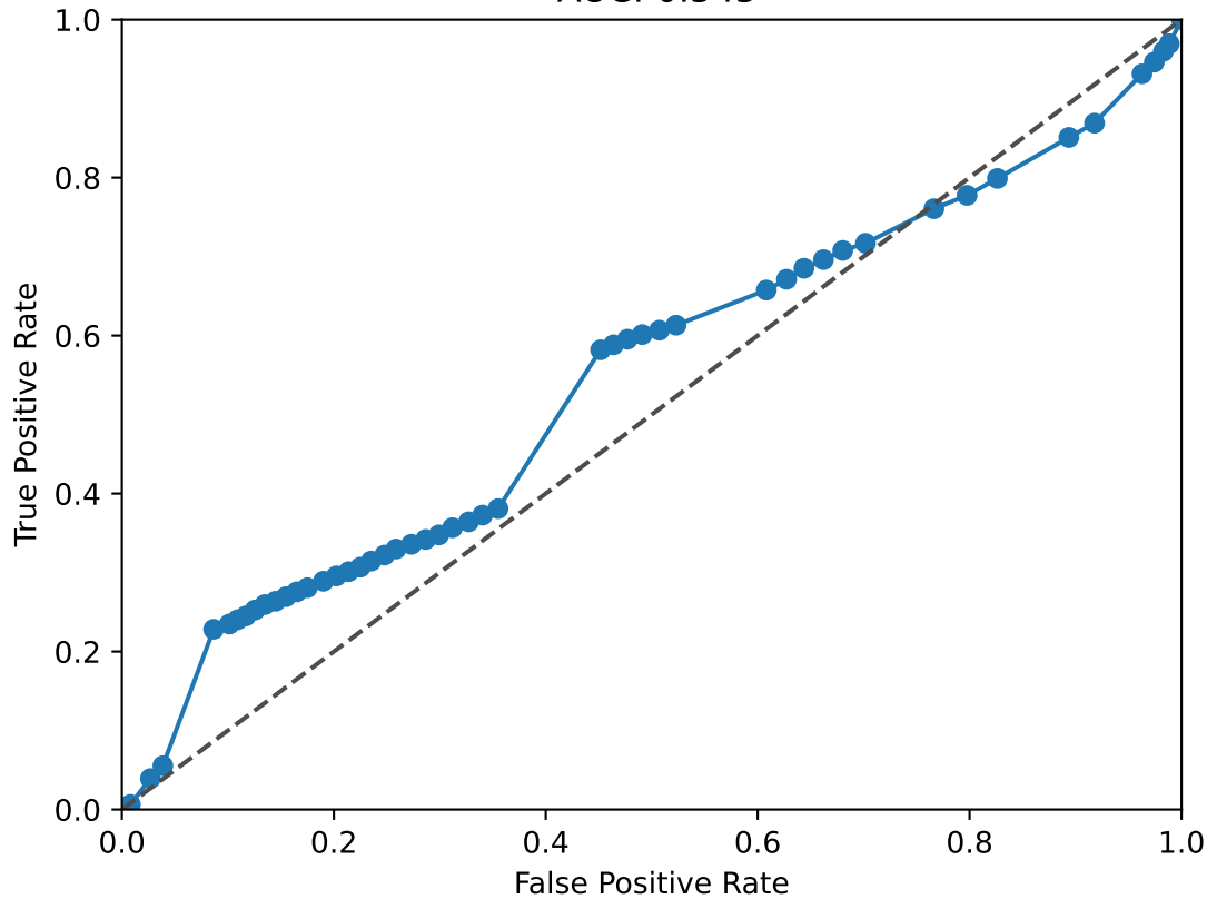
NFKB1 ROC Curve AUC: 0.545
