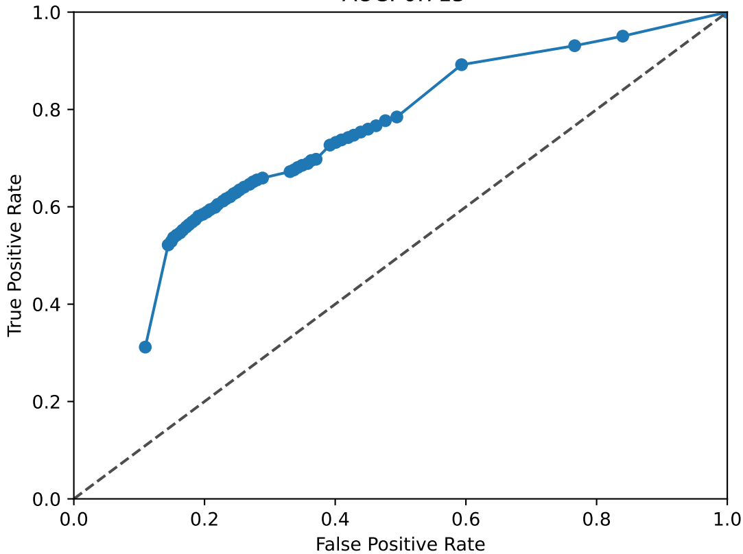
REST ROC Curve AUC: 0.715
