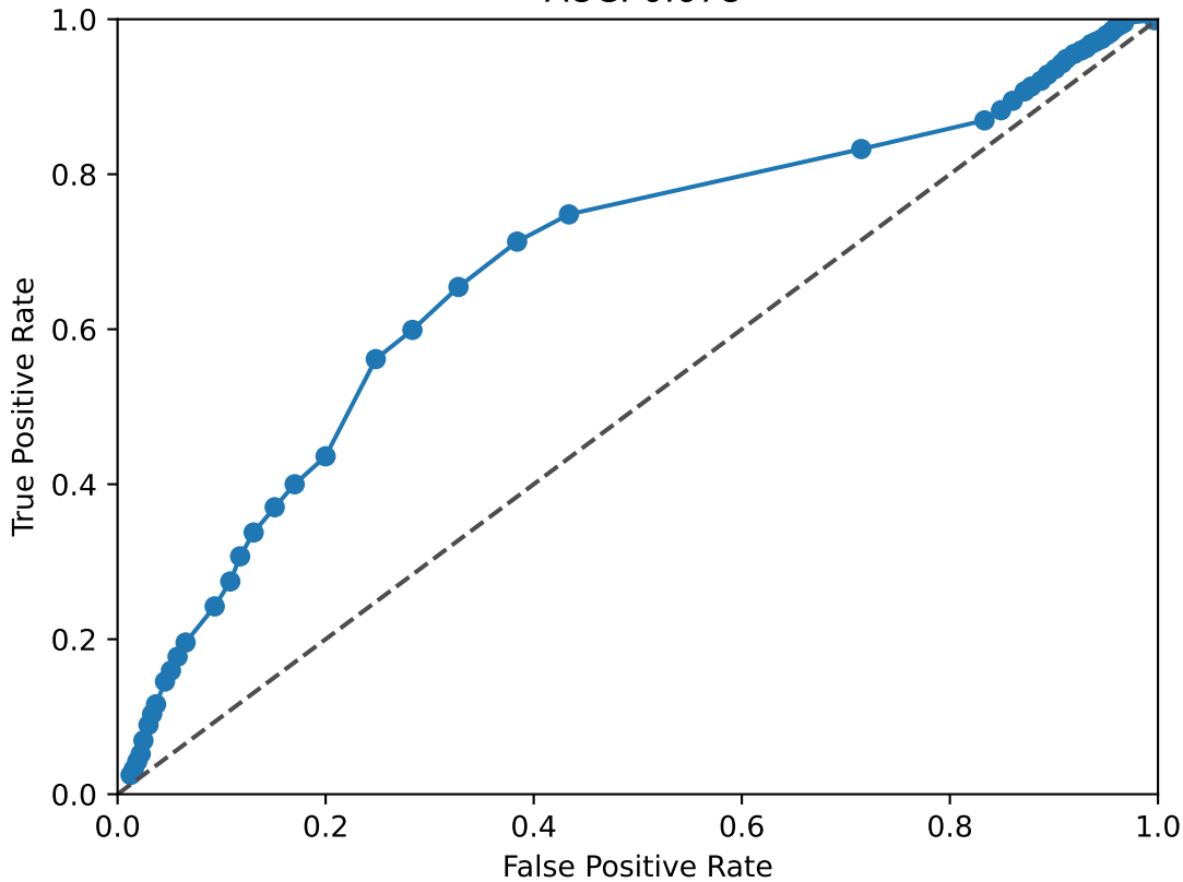
SIX4 ROC Curve AUC: 0.678
